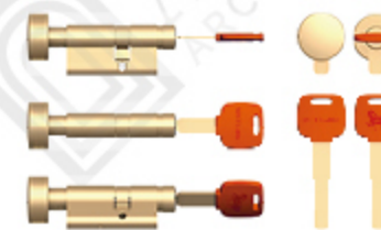
KEY01 super-C combination lock core
